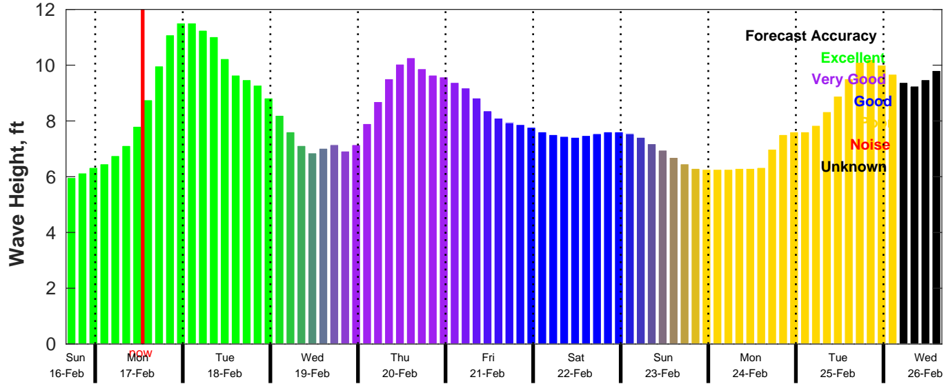
CMEMS Wave Forecast for NDBC 46054 from 16-Feb-2025 16:00:00 to 26-Feb-2025 16:00:00
