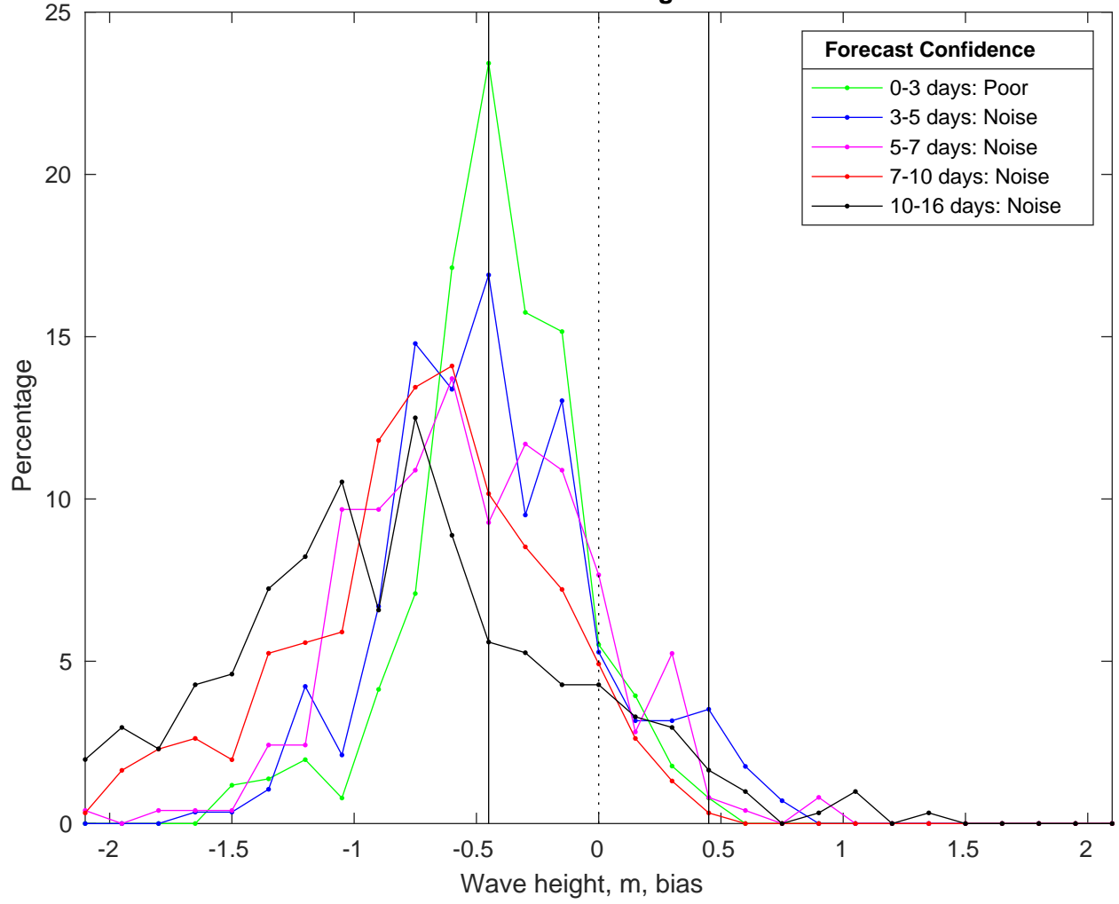
NDBC 46069 vs GFS Waves Bias Histogram: 17-Feb-2025
