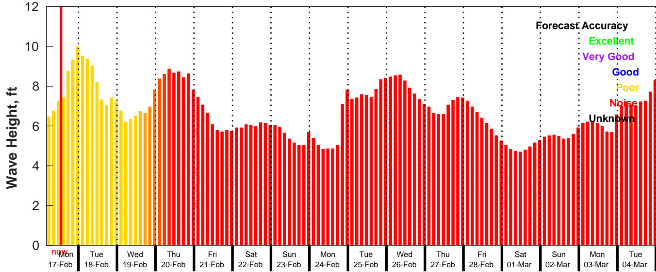
GFS Wave Forecast for NDBC 46069 from 17-Feb-2025 04:00:00 to 05-Mar-2025 04:00:00
