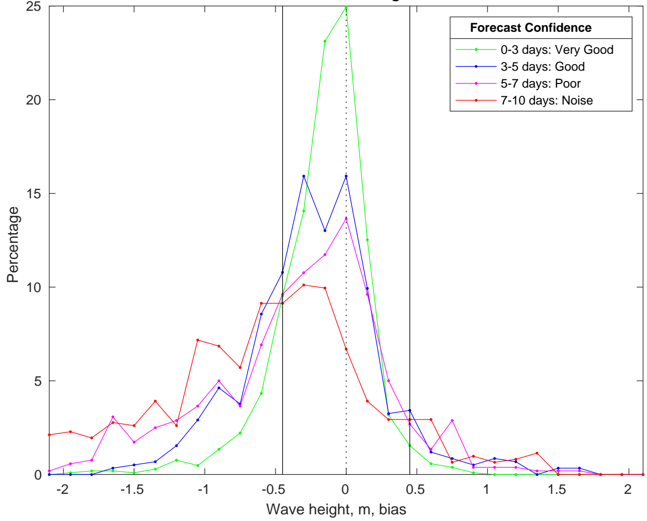
NDBC 46246 vs CMEMS Waves Bias Histogram: 17-Feb-2025
