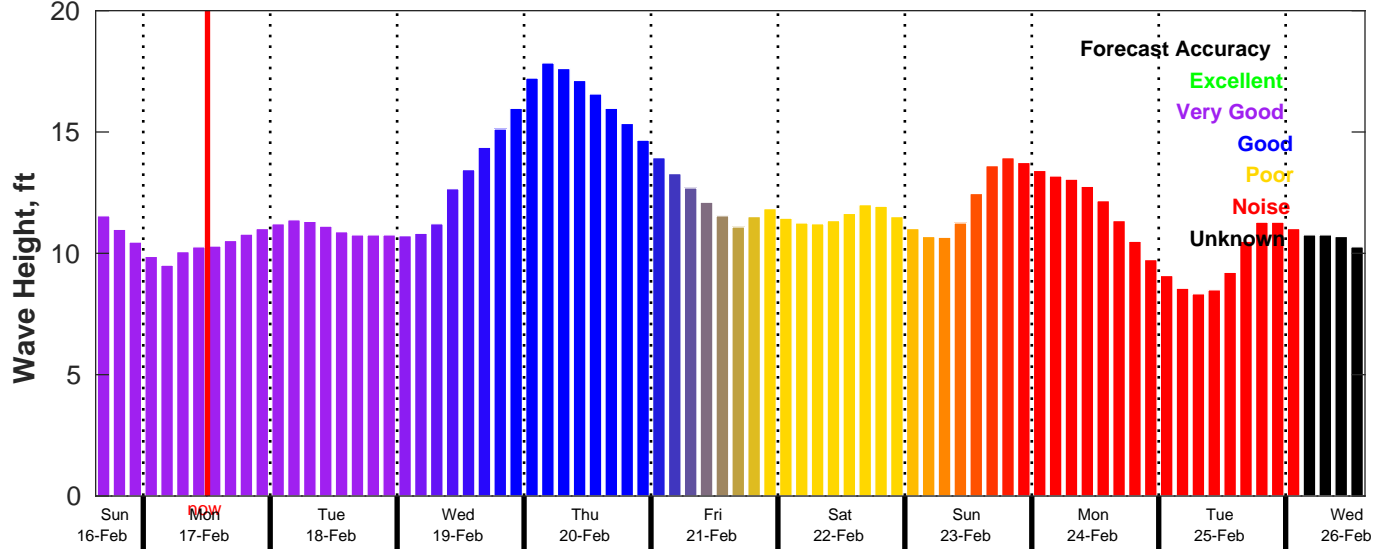
CMEMS Wave Forecast for NDBC 46246 from 16-Feb-2025 15:00:00 to 26-Feb-2025 15:00:00
