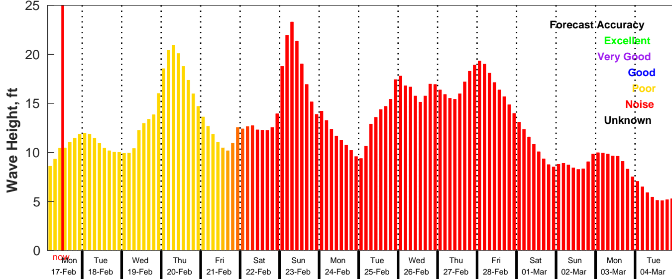
GFS Wave Forecast for NDBC 46246 from 17-Feb-2025 03:00:00 to 05-Mar-2025 03:00:00
