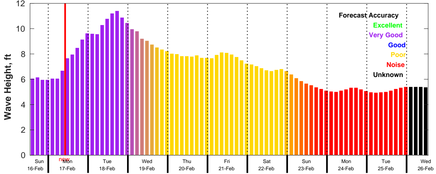
CMEMS Wave Forecast for NDBC 51209 from 16-Feb-2025 13:00:00 to 26-Feb-2025 13:00:00
