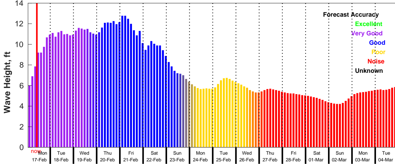
GFS Wave Forecast for NDBC 51209 from 17-Feb-2025 01:00:00 to 05-Mar-2025 01:00:00
