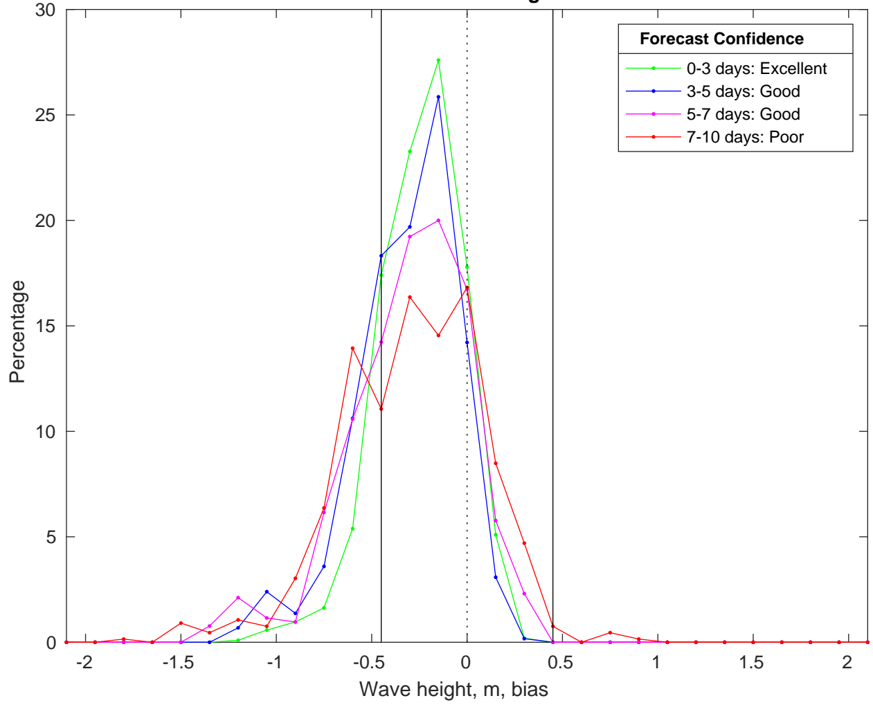
NDBC 52211 vs CMEMS Waves Bias Histogram: 17-Feb-2025
