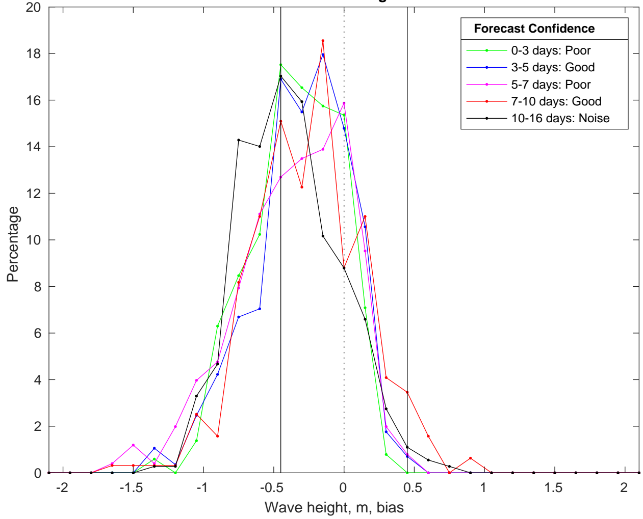
NDBC 52211 vs GFS Waves Bias Histogram: 17-Feb-2025
