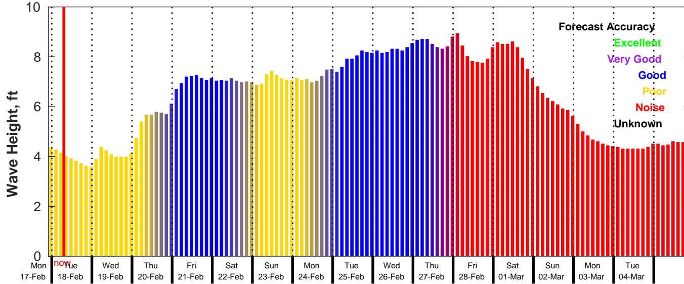
GFS Wave Forecast for NDBC 52211 from 17-Feb-2025 22:00:00 to 05-Mar-2025 22:00:00
