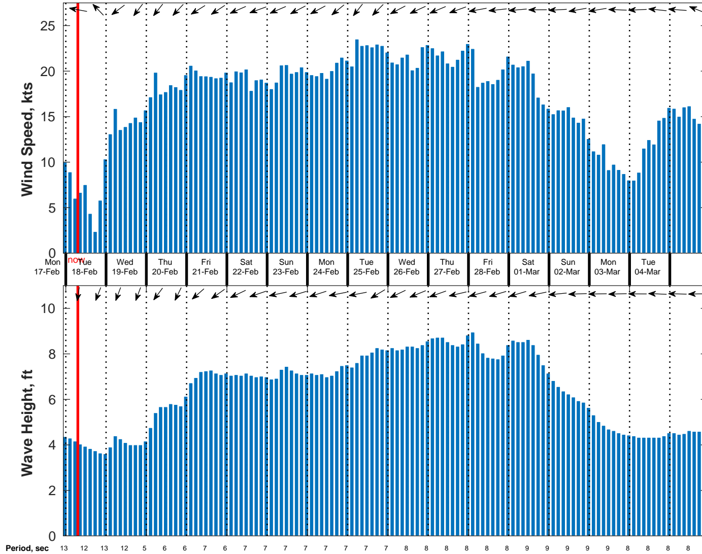
Wind & Wave Forecast for NDBC 52211 from 17-Feb-2025 22:00:00 to 05-Mar-2025 22:00:00
