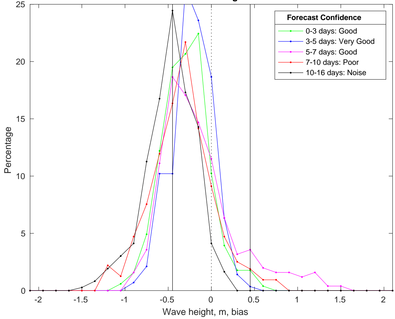
NDBC 52212 vs GFS Waves Bias Histogram: 17-Feb-2025
