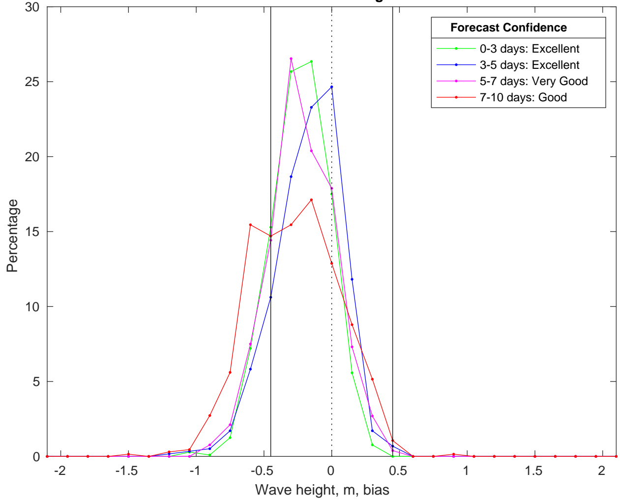
NDBC 52213 vs CMEMS Waves Bias Histogram: 17-Feb-2025
