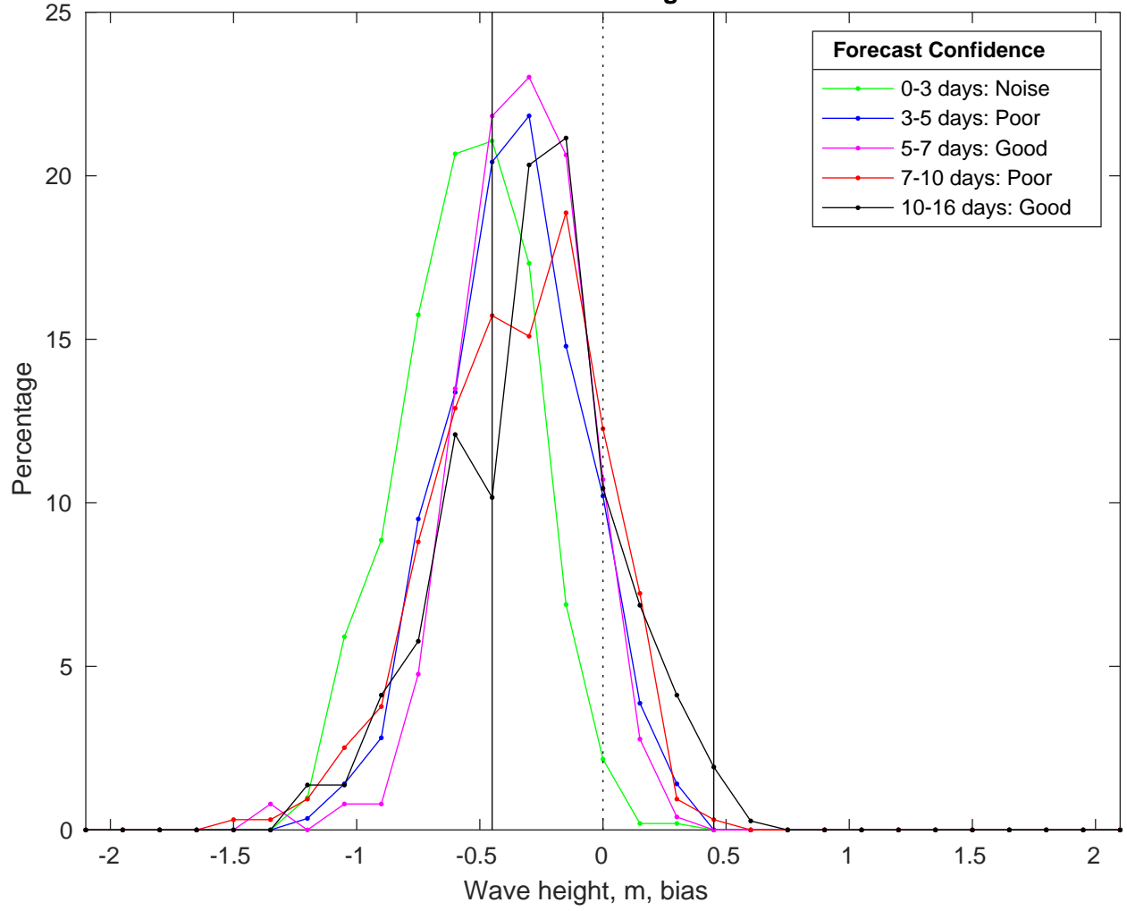
NDBC 52213 vs GFS Waves Bias Histogram: 17-Feb-2025
