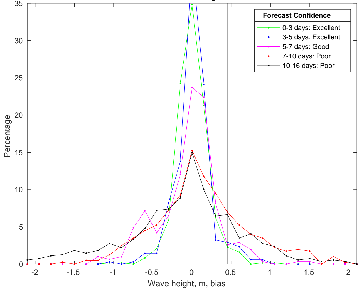
NDBC 41004 vs GFS Waves Bias Histogram: 19-Feb-2025
