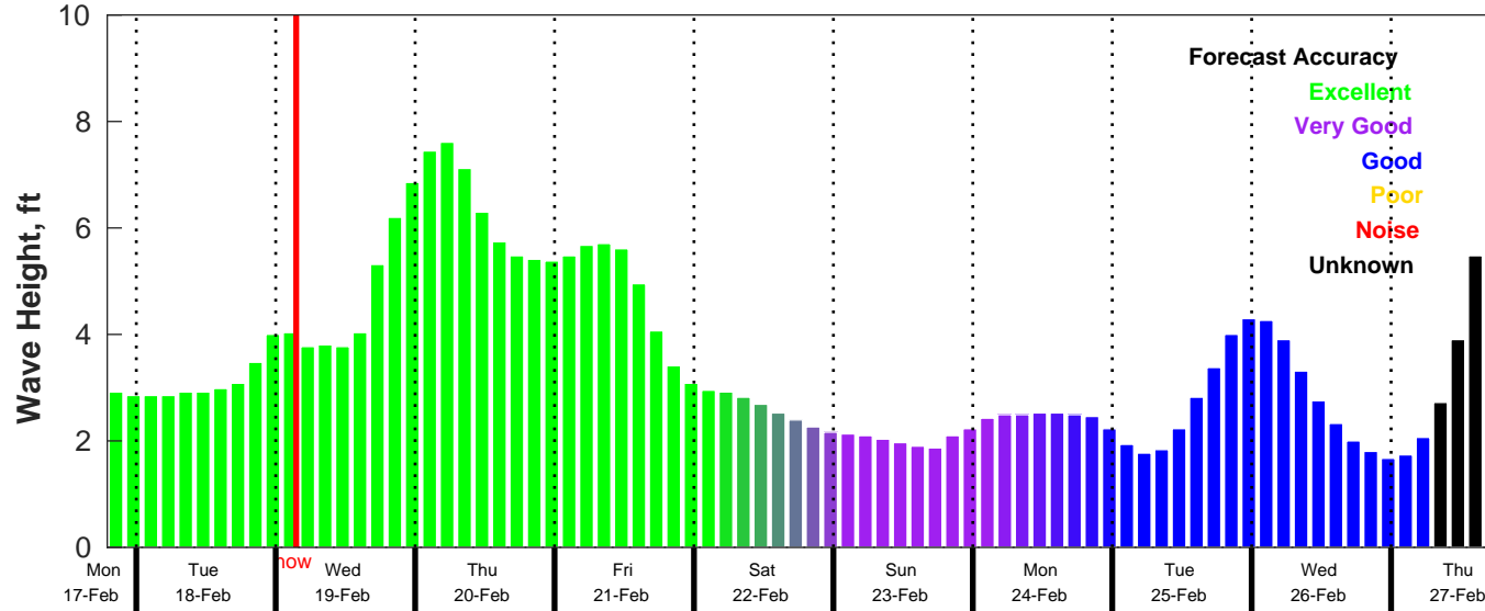
CMEMS Wave Forecast for NDBC 41004 from 17-Feb-2025 19:00:00 to 27-Feb-2025 19:00:00
