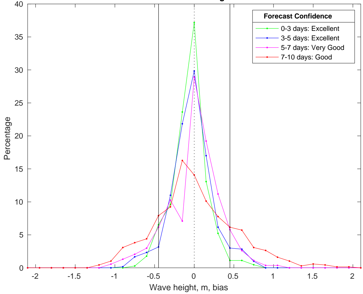
NDBC 41013 vs CMEMS Waves Bias Histogram: 19-Feb-2025
