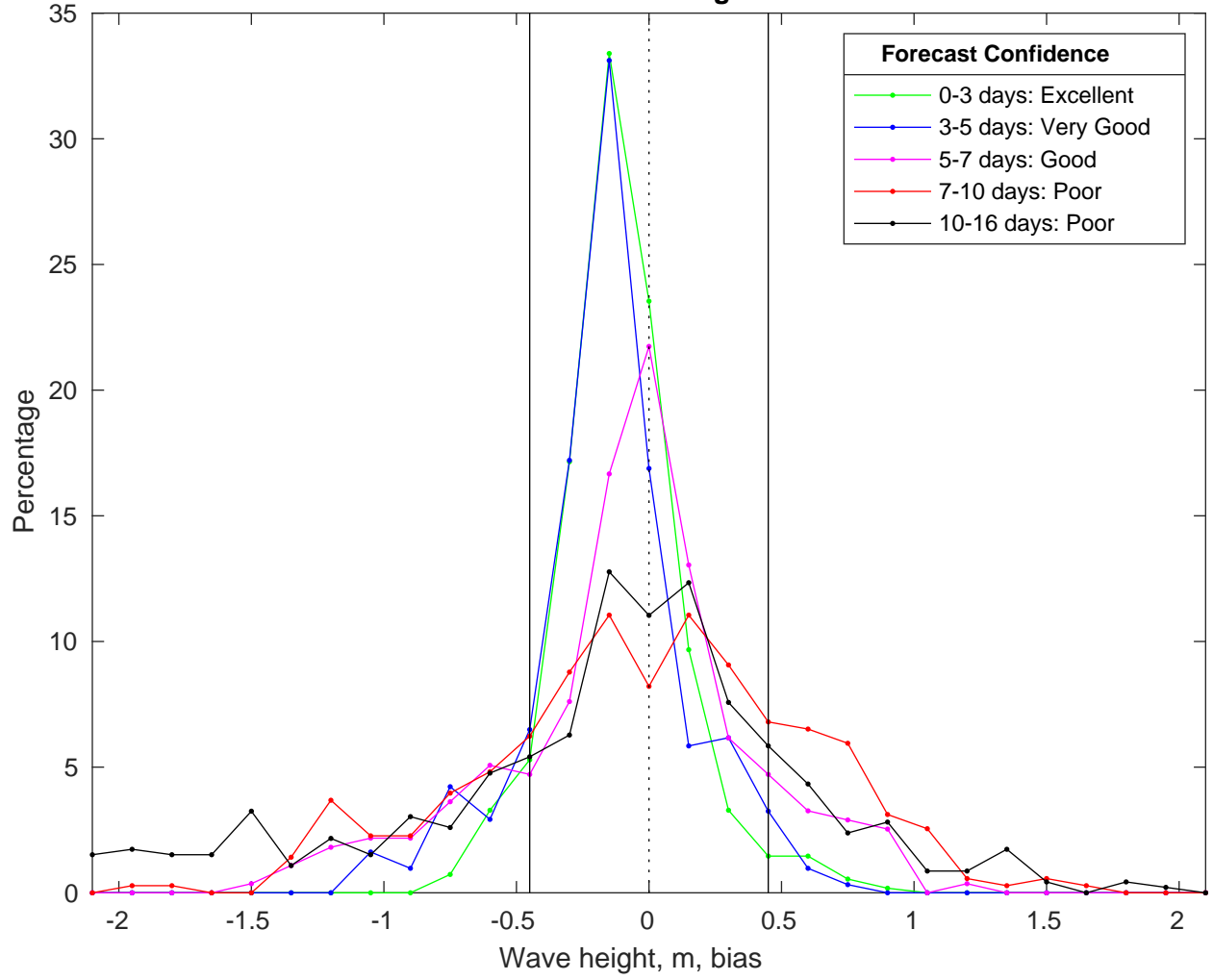
NDBC 41013 vs GFS Waves Bias Histogram: 19-Feb-2025
