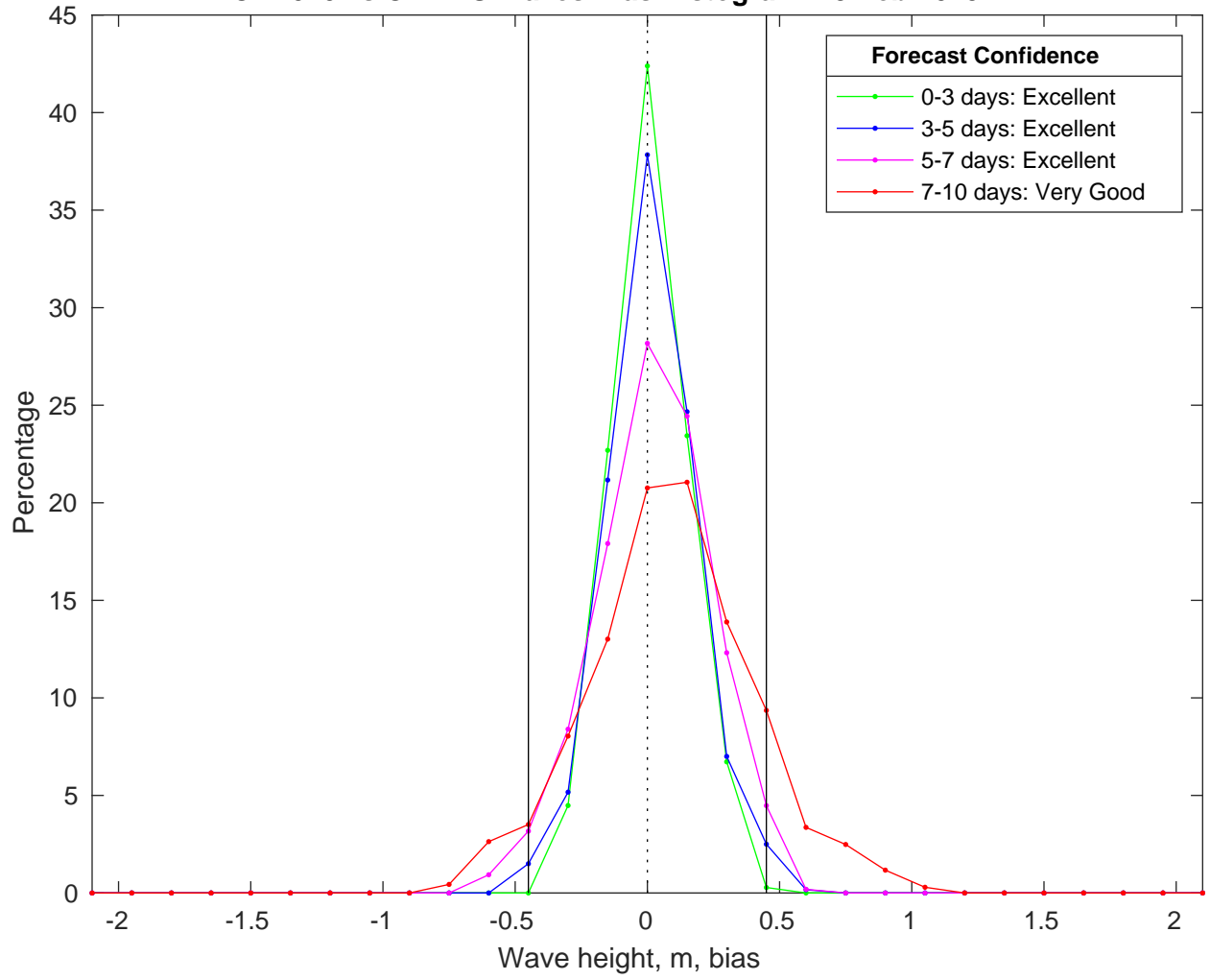
NDBC 41040 vs CMEMS Waves Bias Histogram: 19-Feb-2025
