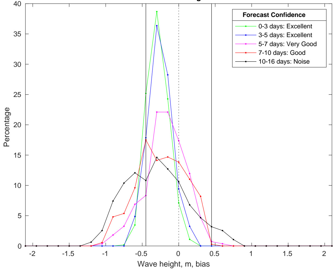
NDBC 41040 vs GFS Waves Bias Histogram: 19-Feb-2025
