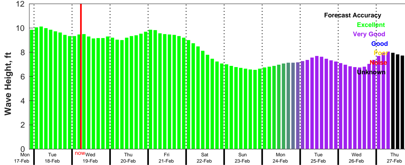
CMEMS Wave Forecast for NDBC 41040 from 17-Feb-2025 21:00:00 to 27-Feb-2025 21:00:00
