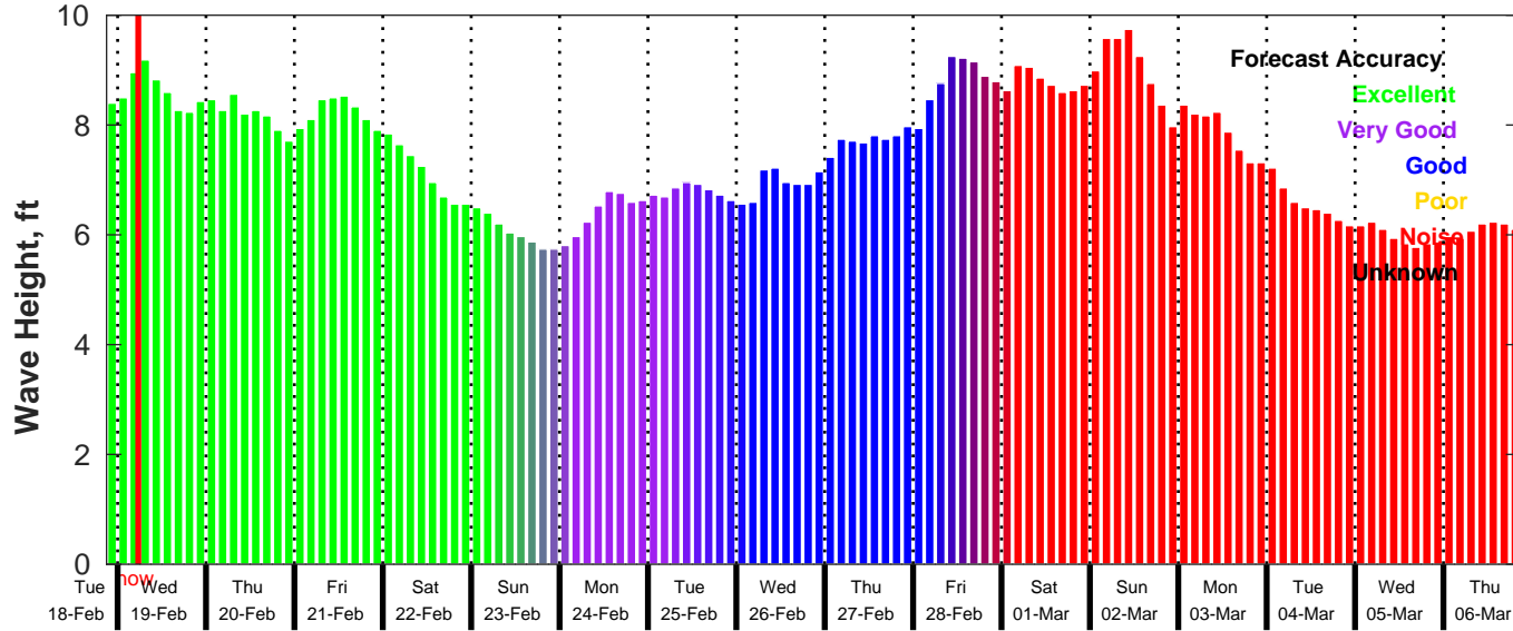
GFS Wave Forecast for NDBC 41040 from 18-Feb-2025 21:00:00 to 06-Mar-2025 21:00:00
