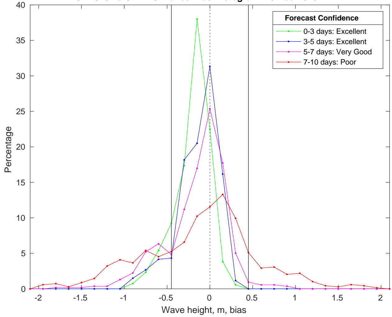
NDBC 42019 vs CMEMS Waves Bias Histogram: 19-Feb-2025
