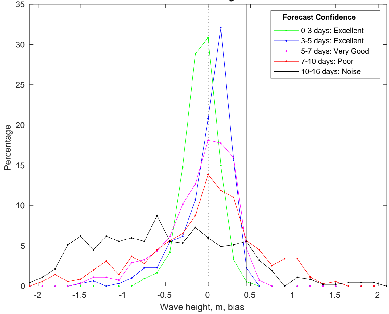
NDBC 42019 vs GFS Waves Bias Histogram: 19-Feb-2025
