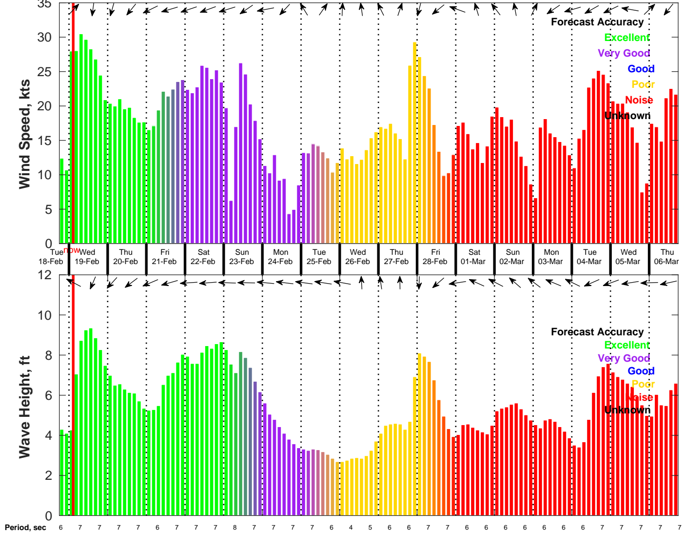
Wind & Wave Forecast for NDBC 42019 from 18-Feb-2025 18:00:00 to 06-Mar-2025 18:00:00
