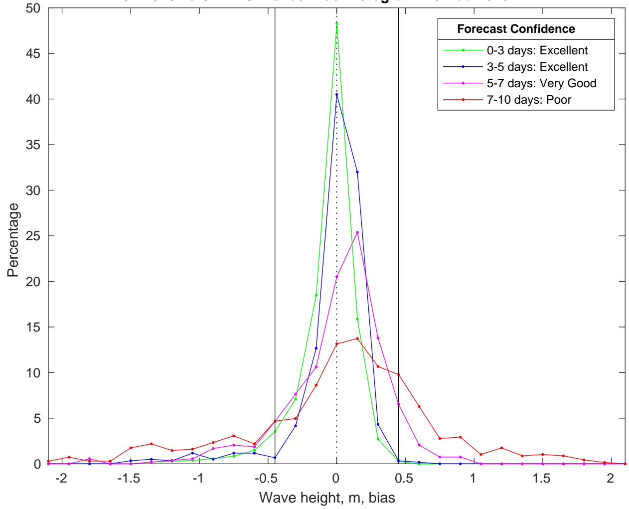
NDBC 42020 vs CMEMS Waves Bias Histogram: 19-Feb-2025
