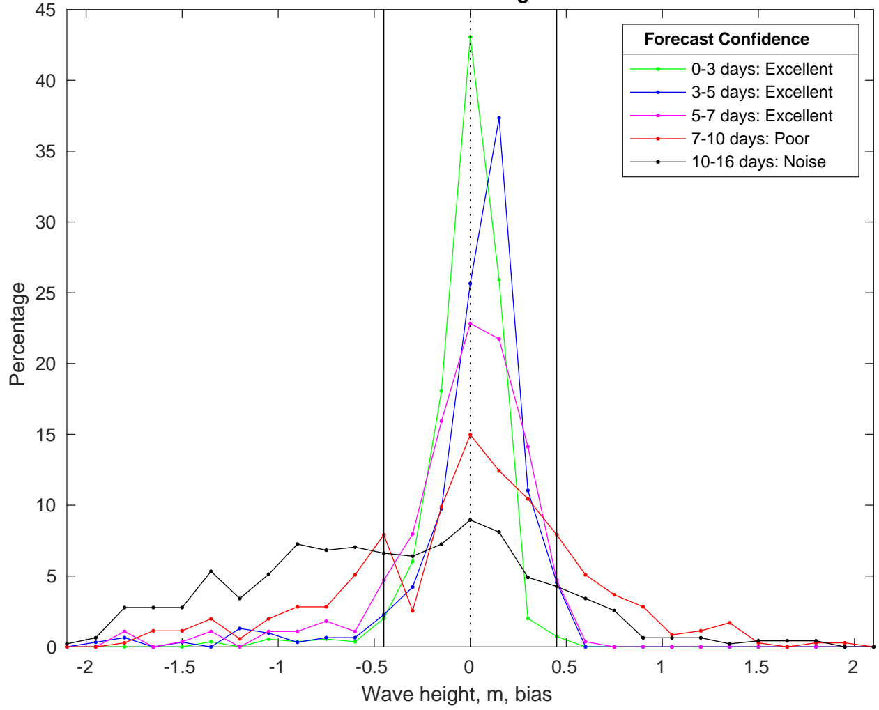
NDBC 42020 vs GFS Waves Bias Histogram: 19-Feb-2025
