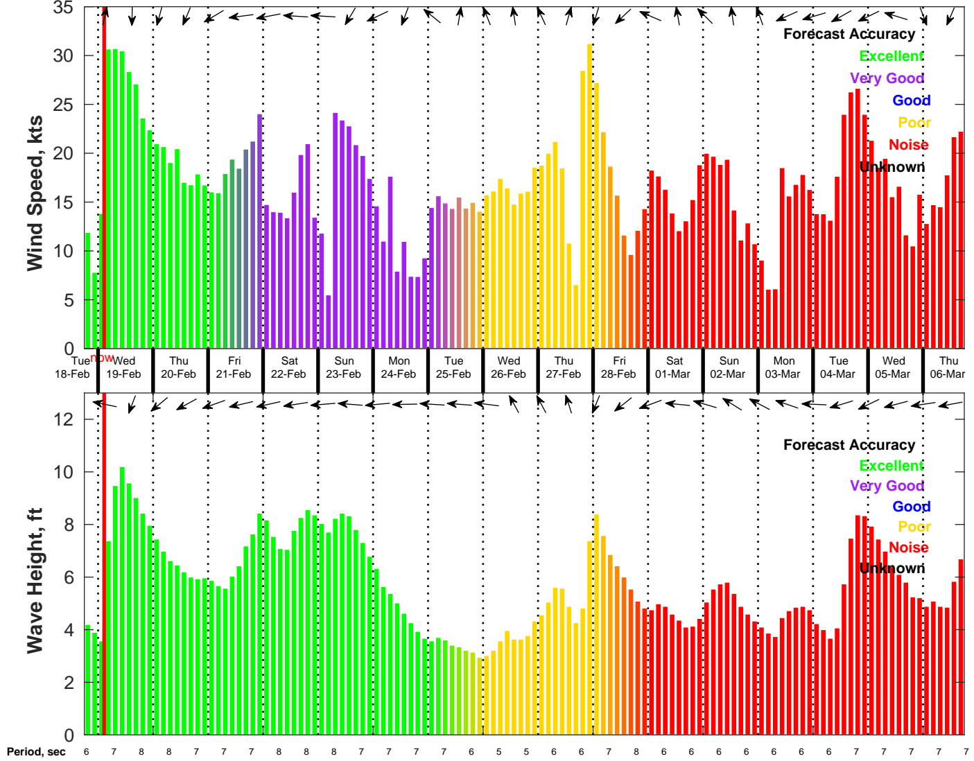
Wind & Wave Forecast for NDBC 42020 from 18-Feb-2025 18:00:00 to 06-Mar-2025 18:00:00
