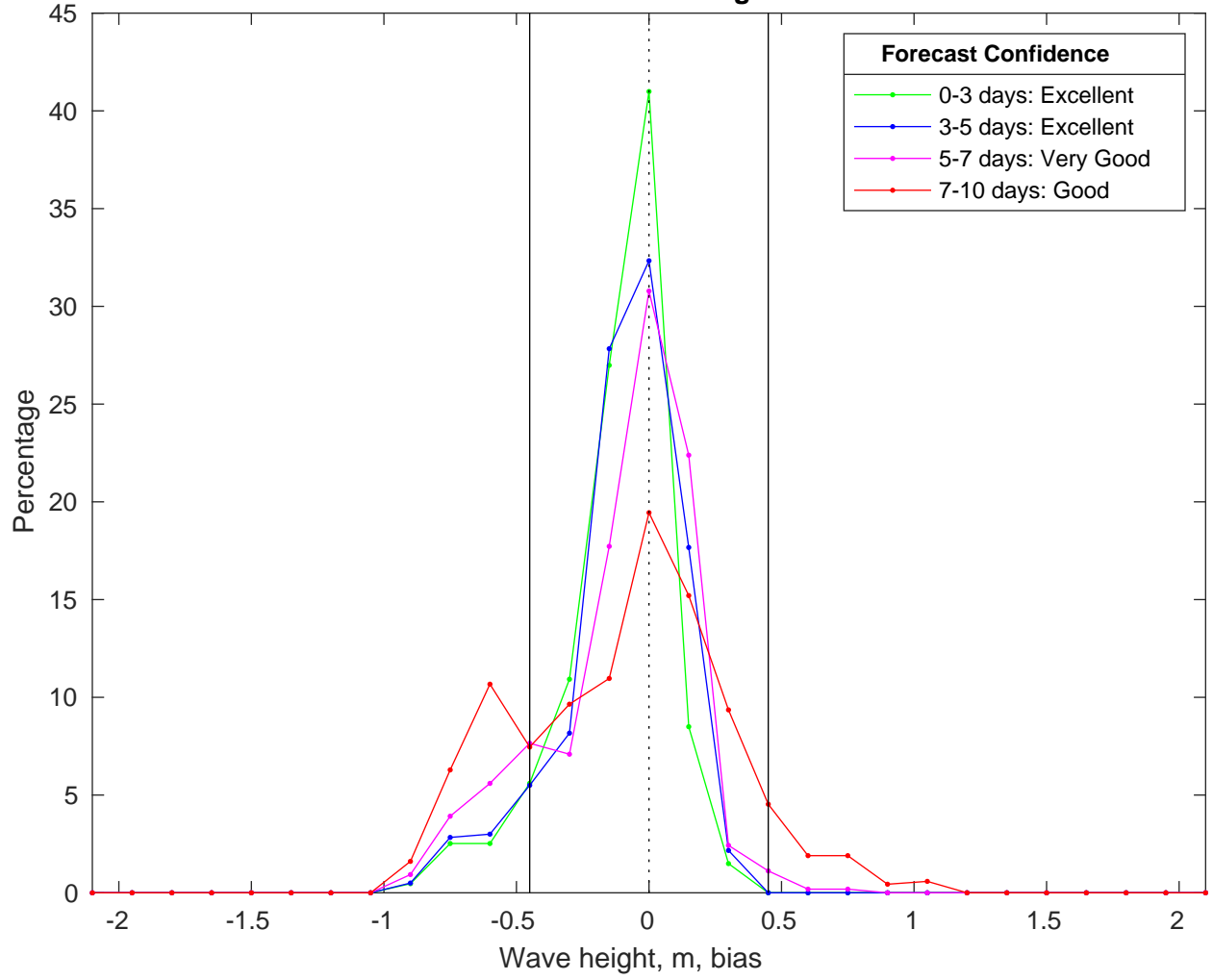
NDBC 42035 vs CMEMS Waves Bias Histogram: 19-Feb-2025
