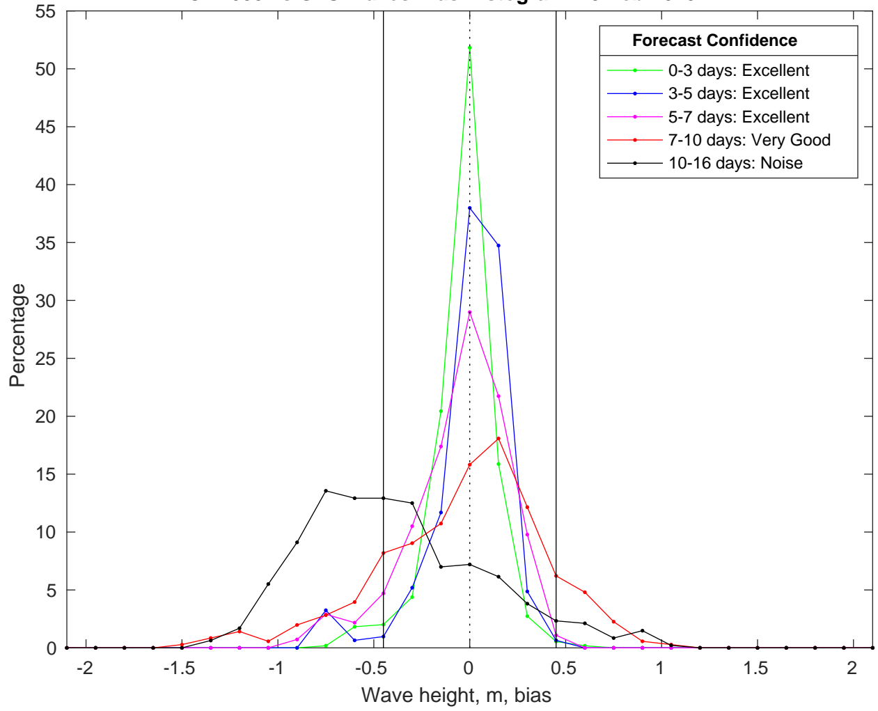
NDBC 42035 vs GFS Waves Bias Histogram: 19-Feb-2025
