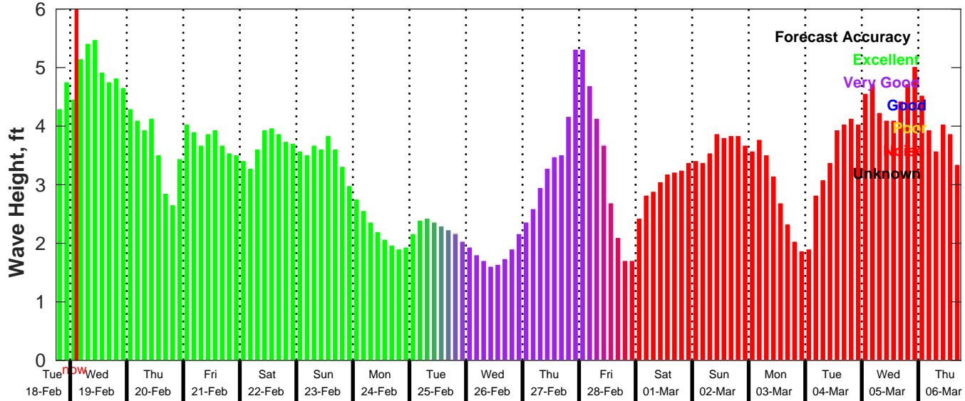
GFS Wave Forecast for NDBC 42035 from 18-Feb-2025 18:00:00 to 06-Mar-2025 18:00:00
