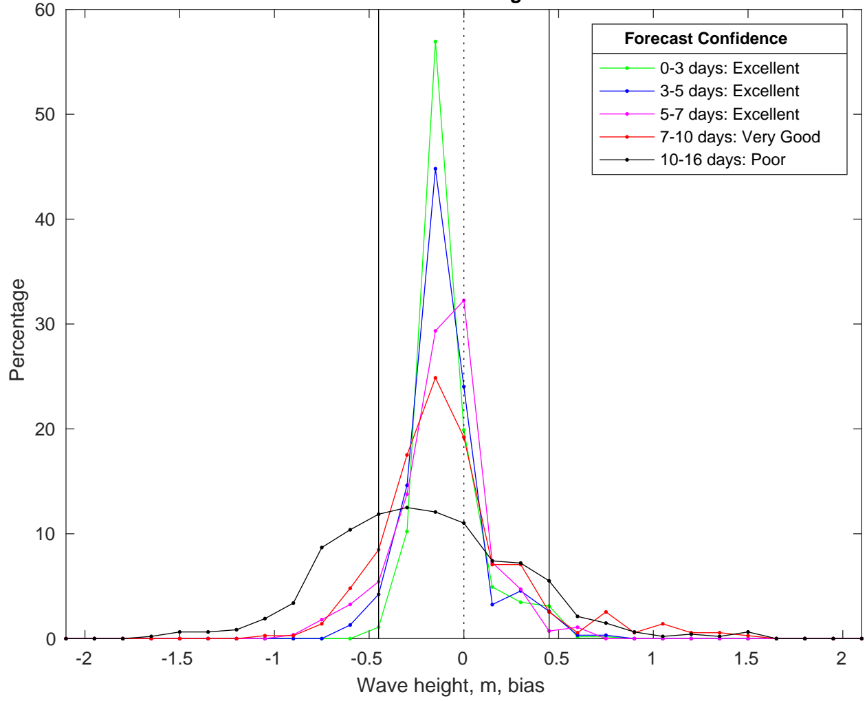
NDBC 42036 vs GFS Waves Bias Histogram: 19-Feb-2025
