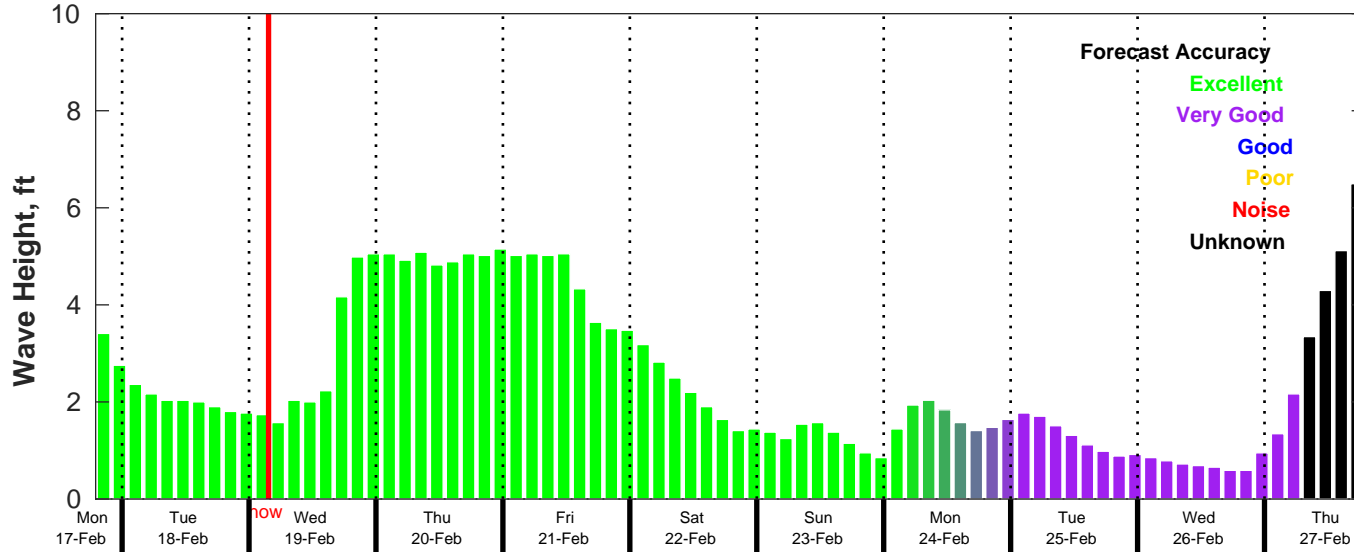
CMEMS Wave Forecast for NDBC 42036 from 17-Feb-2025 19:00:00 to 27-Feb-2025 19:00:00
