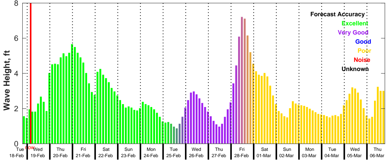
GFS Wave Forecast for NDBC 42036 from 18-Feb-2025 19:00:00 to 06-Mar-2025 19:00:00
