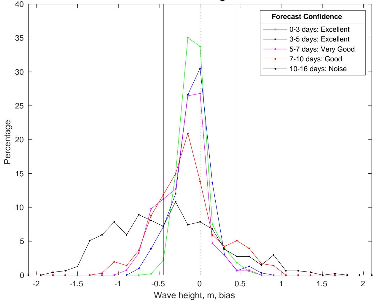
NDBC 42040 vs GFS Waves Bias Histogram: 19-Feb-2025
