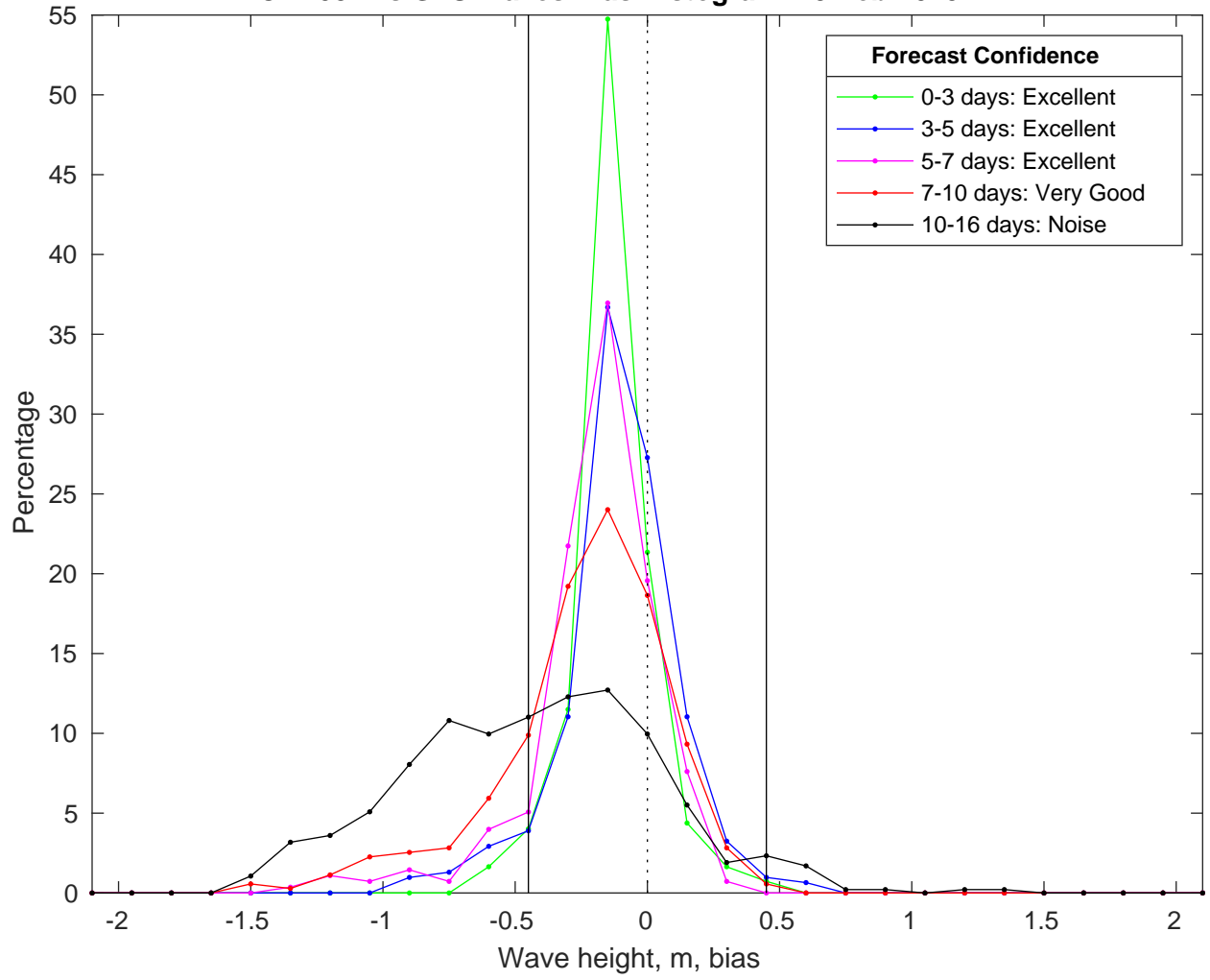
NDBC 42084 vs GFS Waves Bias Histogram: 19-Feb-2025
