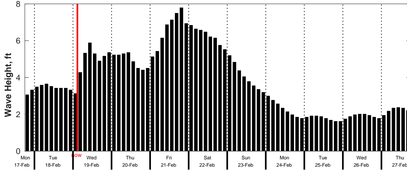
CMEMS Wave Forecast for NDBC 42092 from 17-Feb-2025 18:00:00 to 27-Feb-2025 18:00:00
