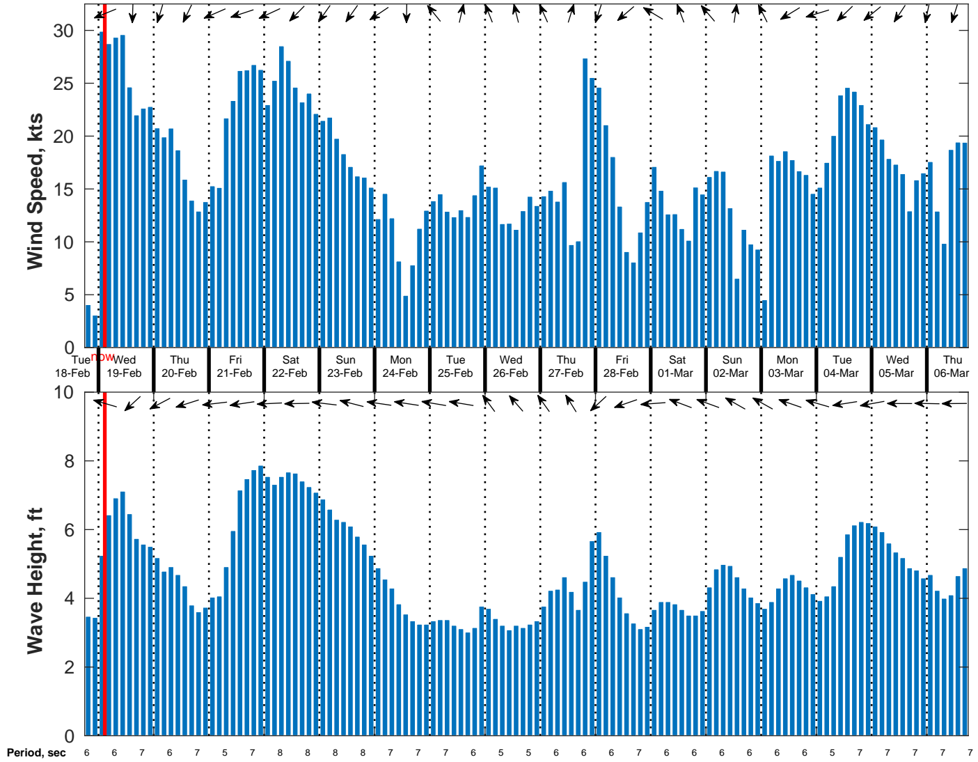
Wind & Wave Forecast for NDBC 42092 from 18-Feb-2025 18:00:00 to 06-Mar-2025 18:00:00
