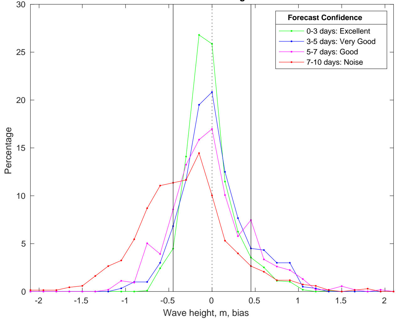
NDBC 46011 vs CMEMS Waves Bias Histogram: 19-Feb-2025
