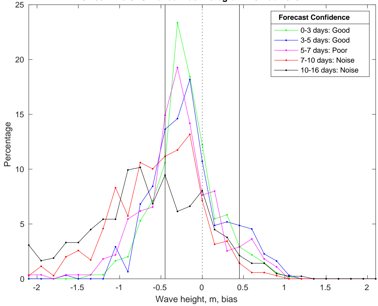
NDBC 46011 vs GFS Waves Bias Histogram: 19-Feb-2025
