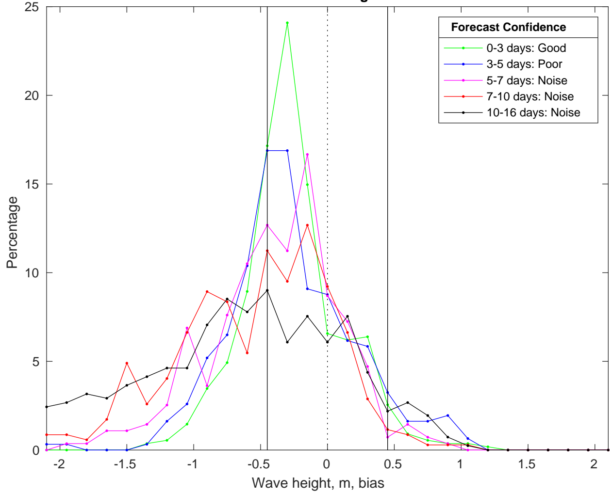
NDBC 46028 vs GFS Waves Bias Histogram: 19-Feb-2025
