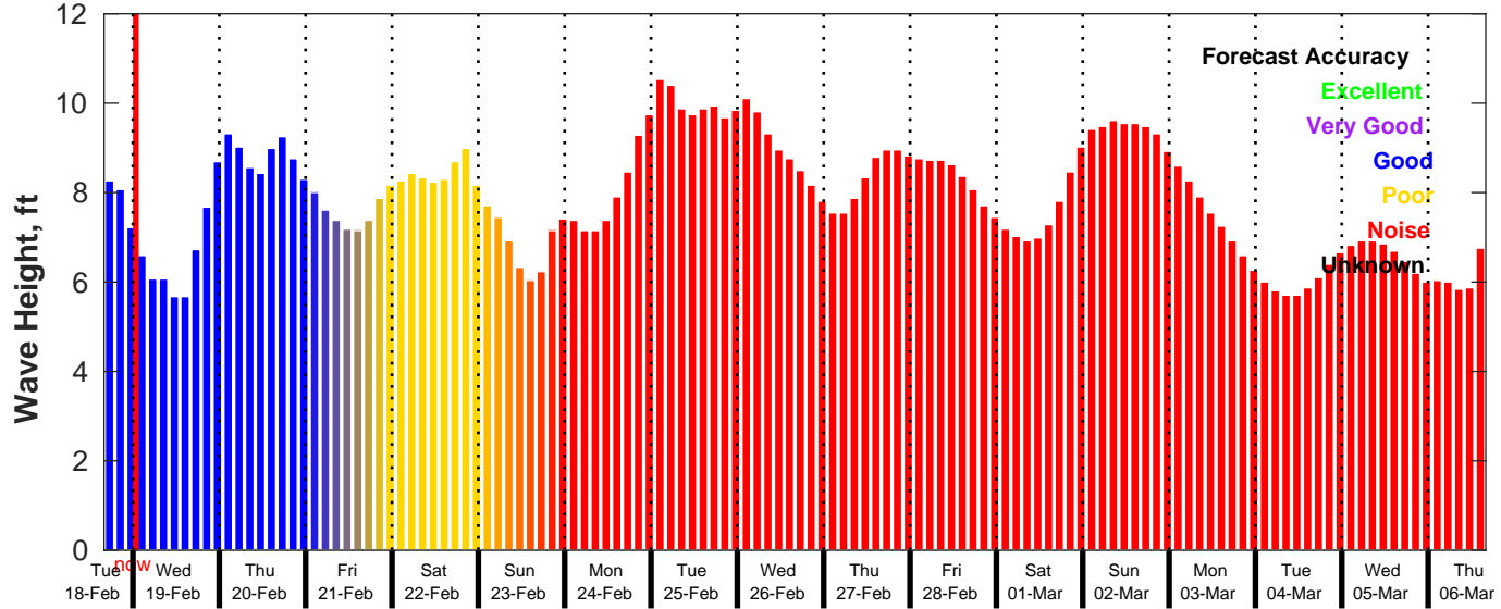
GFS Wave Forecast for NDBC 46028 from 18-Feb-2025 16:00:00 to 06-Mar-2025 16:00:00
