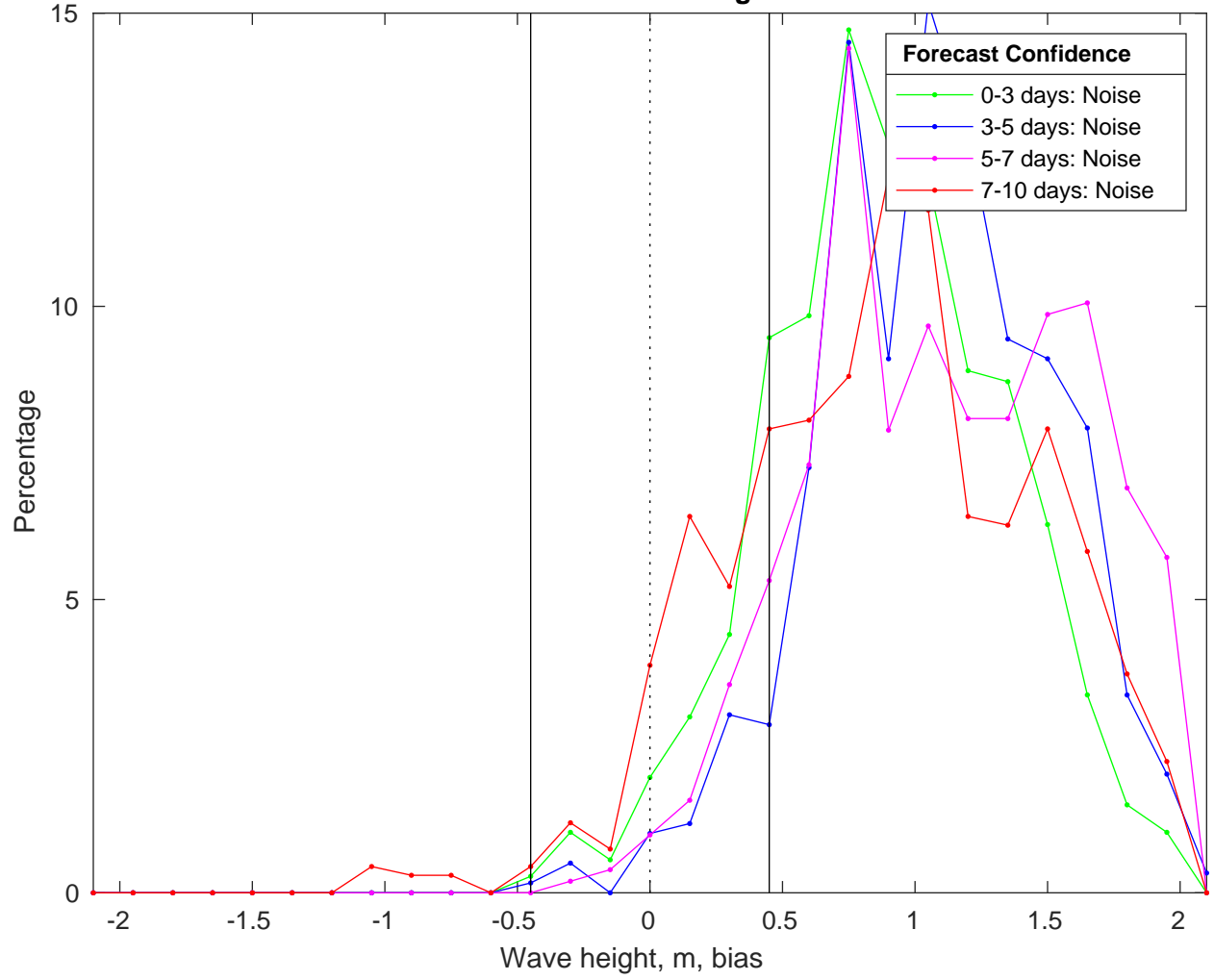
NDBC 46053 vs CMEMS Waves Bias Histogram: 19-Feb-2025
