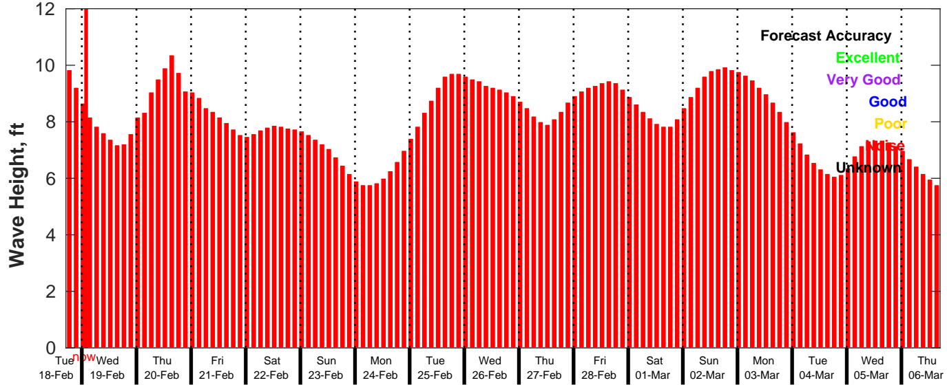
GFS Wave Forecast for NDBC 46053 from 18-Feb-2025 17:00:00 to 06-Mar-2025 17:00:00
