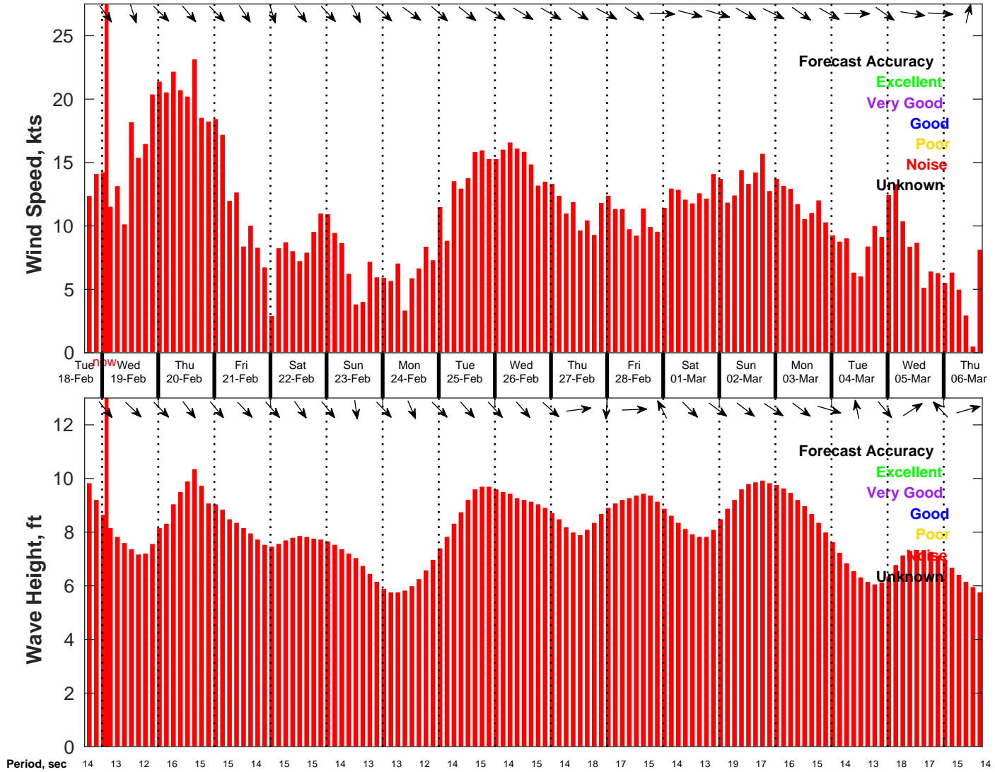
Wind & Wave Forecast for NDBC 46053 from 18-Feb-2025 17:00:00 to 06-Mar-2025 17:00:00
