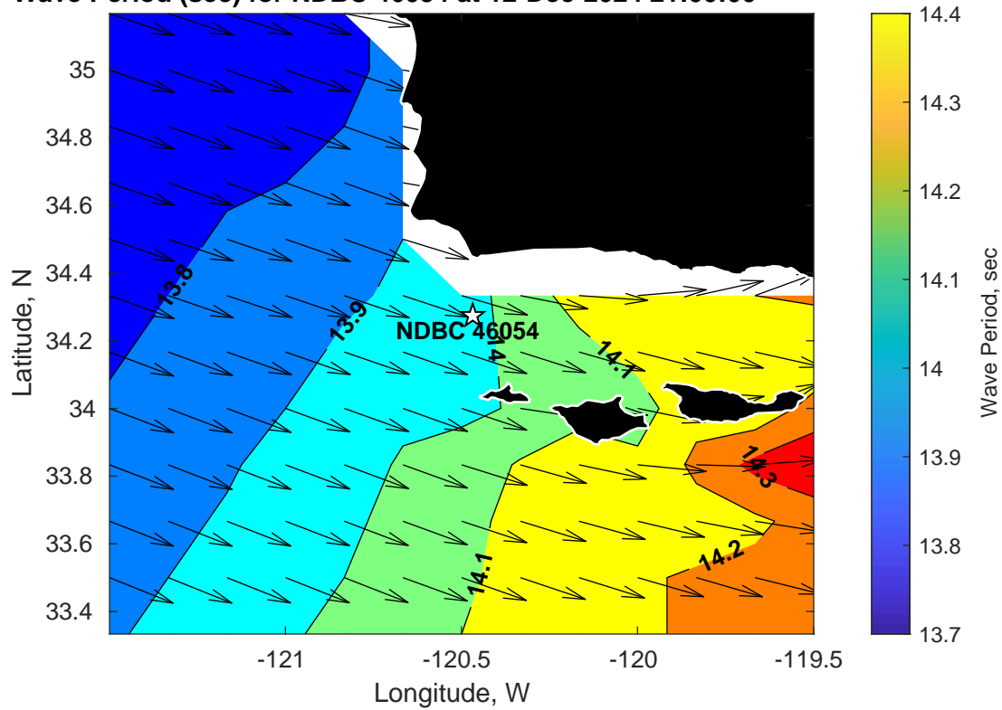
Wave Period (sec) for NDBC 46054 at 12-Dec-2024 21:00:00
