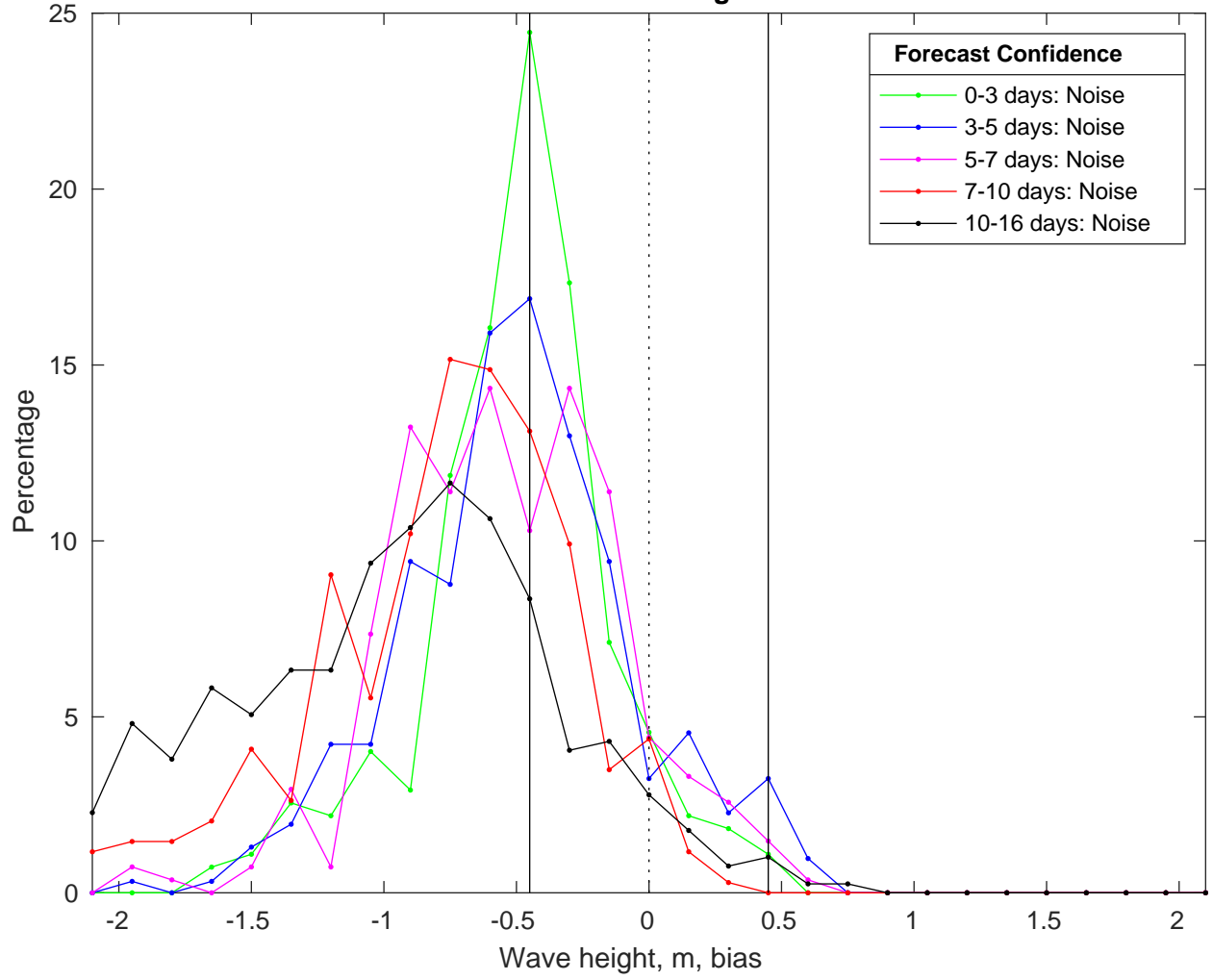
NDBC 46054 vs GFS Waves Bias Histogram: 19-Feb-2025
