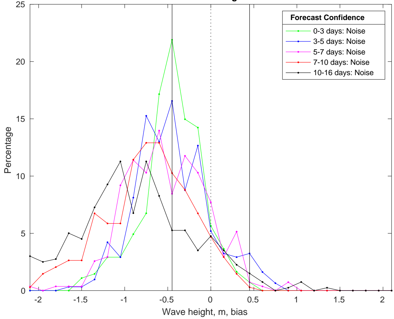
NDBC 46069 vs GFS Waves Bias Histogram: 19-Feb-2025
