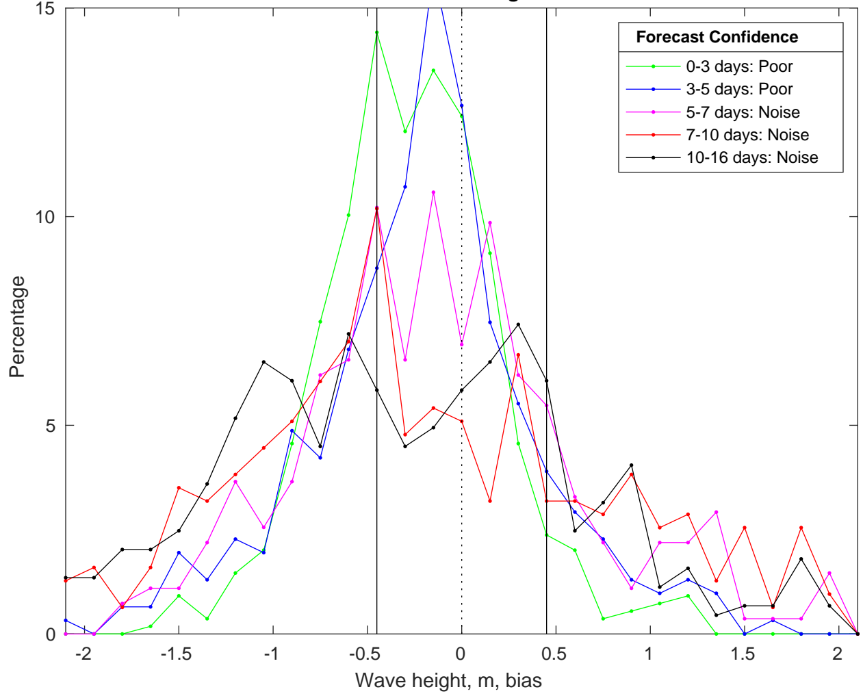
NDBC 46246 vs GFS Waves Bias Histogram: 19-Feb-2025
